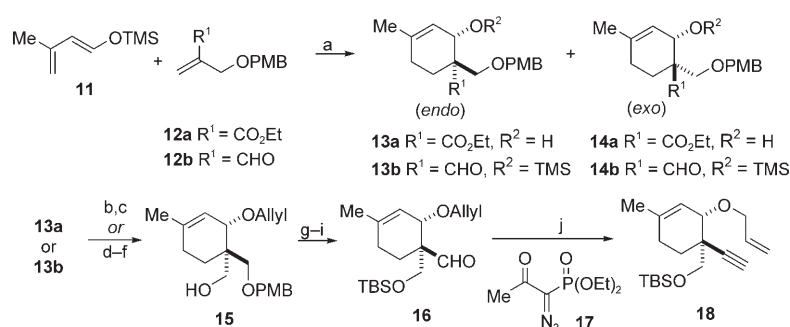
Scheme 2. Reagents and conditions: a) 1) Toluene, 145 °C, 48 h; 2) TBAF, THF, 10 min, 88% ( 13a / 14a = 2:1) or benzene, 80 °C, 22 h, 87% ( 13b / 14b = 6:1); b) allyl bromide, NaH, TBAI, HMPA, THF, 0 °C to 23 °C, 85%; c) DIBAL, CH 2 Cl 2 , 0 °C, 100% (from 13a ); d) NaClO 2 , NaH 2 PO 4 ·H 2 O, t BuOH, H 2 O, 2-methyl-2-butene, 99%; e) allyl bromide, NaH, TBAI, HMPA, THF, 61% (+8% diastereomer); f) DIBAL, CH 2 Cl 2 , 0 °C, 100% (from 13b ); g) TBSCl, imid, CH 2 Cl 2 , 100%; h) DDQ, CH 2 Cl 2 , 84%; i) DMSO, (COCl) 2 , Et 3 N, CH 2 Cl 2 , –78 °C to 0 °C, 90%; j) 17 , K 2 CO 3 , MeOH, 85%. TMS = trimethylsilyl; PMB = p -methoxybenzyl; TBAF = tetra- n -butylammonium fluoride; TBAI = tetra- n -butylammonium iodide; HMPA = hexamethylphosphoramide; DIBAL = diisobutylaluminum hydride; TBS = tert -butyldimethylsilyl; imid = imidazole; DDQ = 2,3-dichloro-5,6-dicyanobenzoquinone; DMSO = dimethyl sulfoxide.
