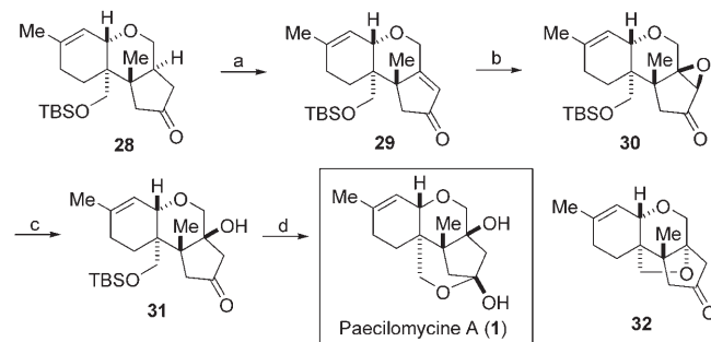
Scheme 6. Reagents and conditions: a) 1) \text{LiTMP} , \text{TMSCl} , THF, -78^\circ\text{C} \rightarrow 0^\circ\text{C} ; 2) \text{Pd}(\text{OAc})_2 , \text{CH}_3\text{CN} , 68% (71% brsm); b) aq. \text{H}_2\text{O}_2 , 6N \text{NaOH} , MeOH, 0^\circ\text{C} , 83% (89% brsm); c) \text{Li} , \text{NH}_3 , THF, -33^\circ\text{C} , 63% (24% 29 ); d) \text{HF}/\text{CH}_3\text{CN} (5:95), 86%. TMP = 2,2,6,6-tetramethylpiperidine.
