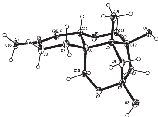
Figure 1. ORTEP representation of paecilomycine A ( 1 ) with ellipsoids shown at the 20% probability level.
