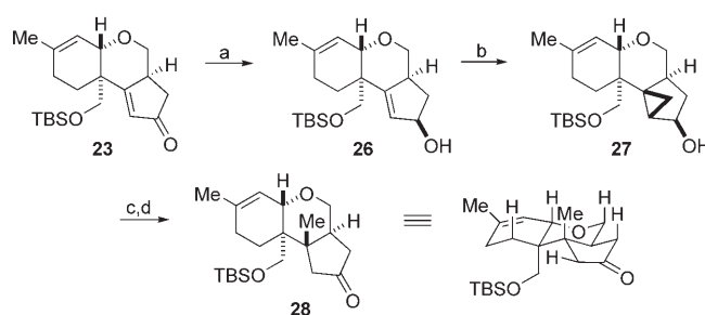
Scheme 5. Reagents and conditions: a) \text{NaBH}_4 , \text{CeCl}_3 \cdot 7\text{H}_2\text{O} , MeOH, 86% (8% \alpha -alcohol); b) n\text{BuLi} , \text{Et}_2\text{O} , -20^\circ\text{C} and then \text{Et}_2\text{Zn} , \text{CH}_2\text{I}_2 , benzene, 53% (11% 26 + 4% bis-cyclopropane); c) TPAP, NMO, 4-Å M.S., \text{CH}_2\text{Cl}_2 , 93%; d) \text{Li} , \text{NH}_3 , THF, -33^\circ\text{C} , 65% (75% brsm). TPAP = tetra- n -propylammonium perruthenate; NMO = N -methylmorpholine N -oxide; brsm = based on recovered starting material.
