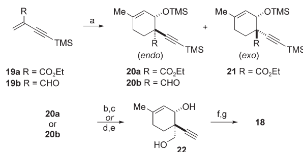
Scheme 3. Reagents and conditions: a) 11 , CH 2 Cl 2 , 23 °C, 3 h, 86% ( endo/exo > 10:1) or 11 , CH 2 Cl 2 , 0 °C, 0.5 h, 58% ( endo/exo > 20:1); b) LiAlH 4 , THF, 0 °C; c) K 2 CO 3 , MeOH, (85% two steps from 20a ); d) NaBH 4 , MeOH, 0 °C; e) K 2 CO 3 , MeOH, (72% two steps from 20b ); f) TBSCl, imid, CH 2 Cl 2 , 89%; g) allyl bromide, NaH, DMF, 70%. DMF = N,N -dimethylformamide.
