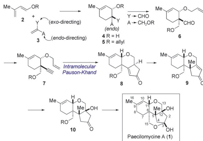
Scheme 1. Synthetic strategy toward paecilomycine A ( 1 ).
