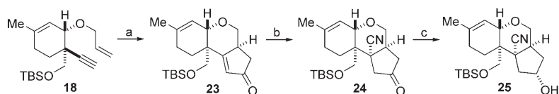
Scheme 4. Reagents and conditions: a) [\text{Co}_2(\text{CO})_8] , 4-Å M.S., toluene, 23°C, 2 h, then 100°C, 24 h, 37%; b) \text{Et}_2\text{AlCN} , toluene, 63%; c) \text{NaBH}_4 , MeOH, 80%.
